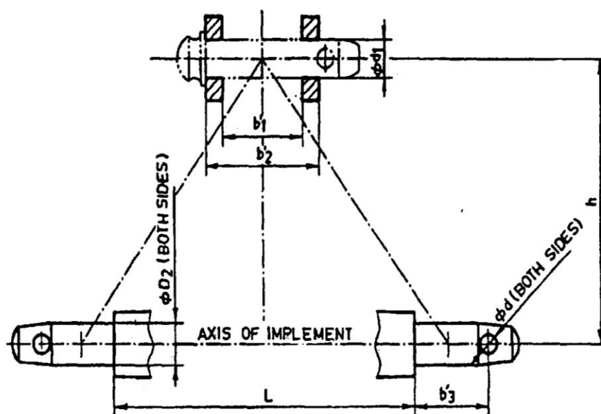
Fig. : Implement Hitch Attachment
